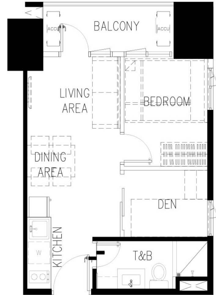
1 Bedroom Unit with Den and Balcony (Suggested Furniture Unit) ± 34.91 sqm
